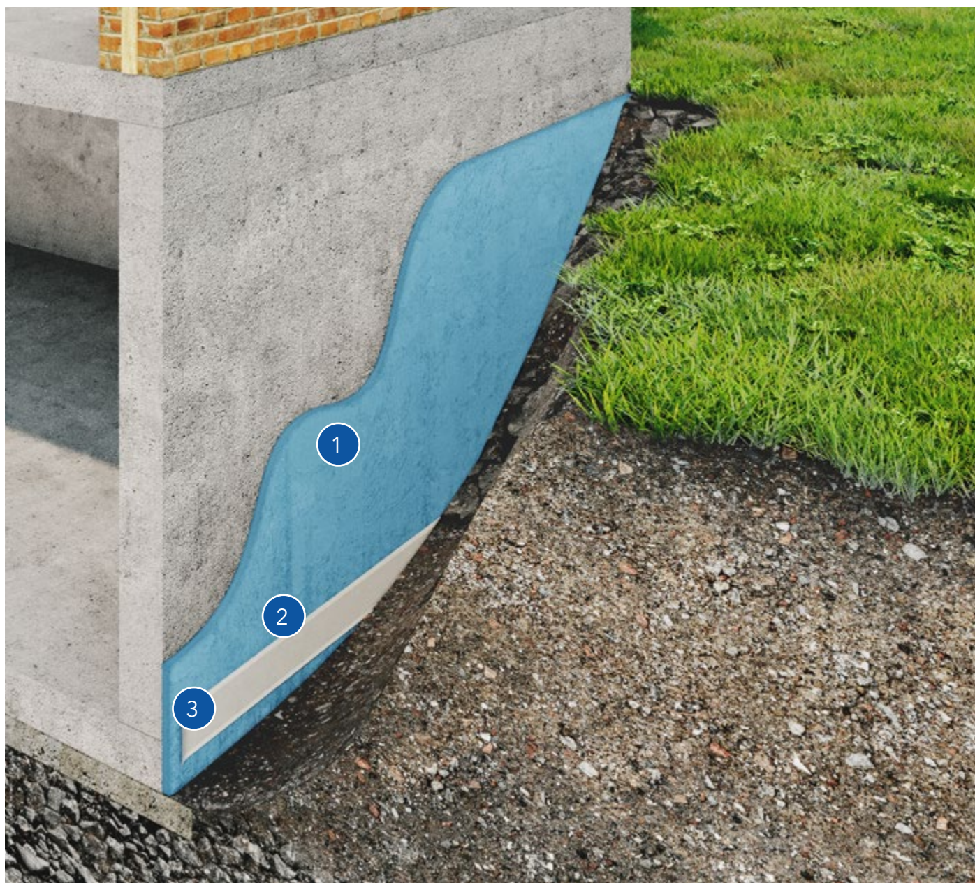
BELOW GROUND CONCRETE WALL AND SLAB - EXTERNAL WATERPROOFING
